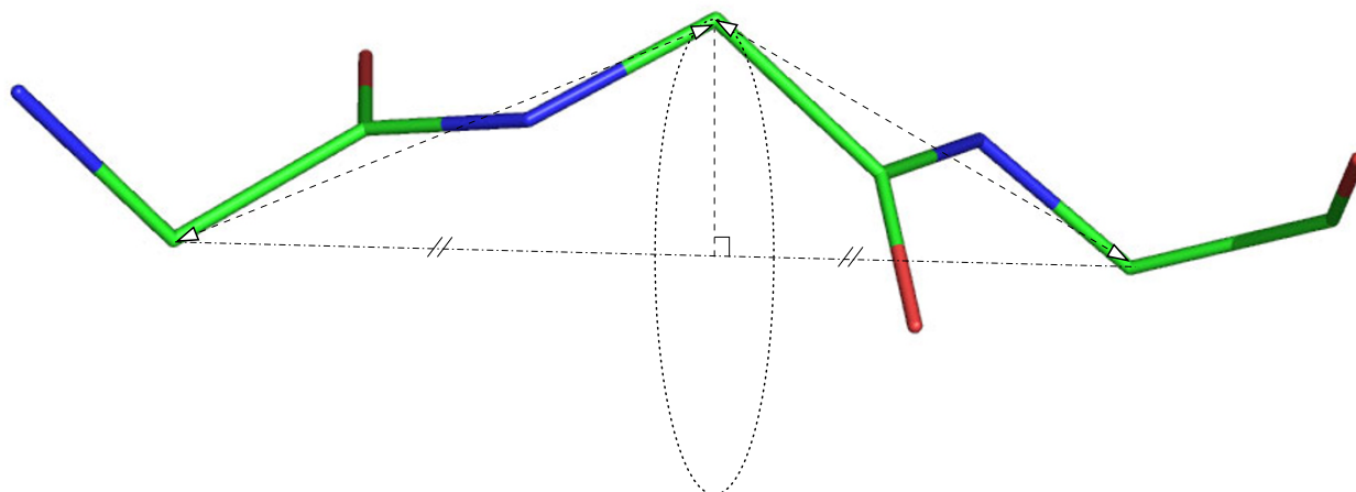
Figure 8 Loop closure procedure in Rappertk . C_{\alpha}^i lies on a circle centered at the mid-point of line joining C_{\alpha}^{j-1} and C_{\alpha}^{j+1} . Radius of the circle is determined by length of the line. The circle is in a plane perpendicular to the line. Candidate C_{\alpha}^j positions are sampled on this circle and \{r, \alpha, \theta\} - \{\varphi, \psi, \omega\} mapping (explained earlier in relation to guided sampling) is used to select a position.
