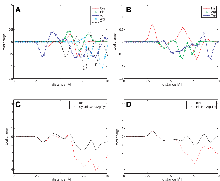
Figure 1 RDF of total charge. The line indicates the distances contributing to each catalytic residue peak for (A) the C4N atom of NAD in 1dc6 and (B) the FE atom of HEM in 1sog (PDB) and to each peak of degenerated catalytic residues and the RDFs for (C) 1dc6 and (D) 1sog (PDB).
